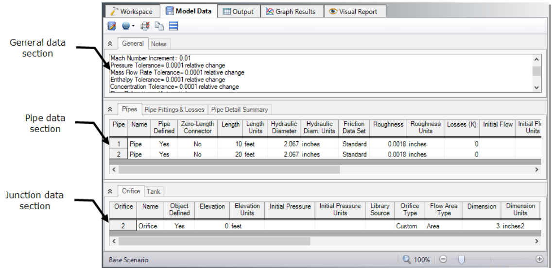
Figure 2.12 The Model Data window shows all input in table form
