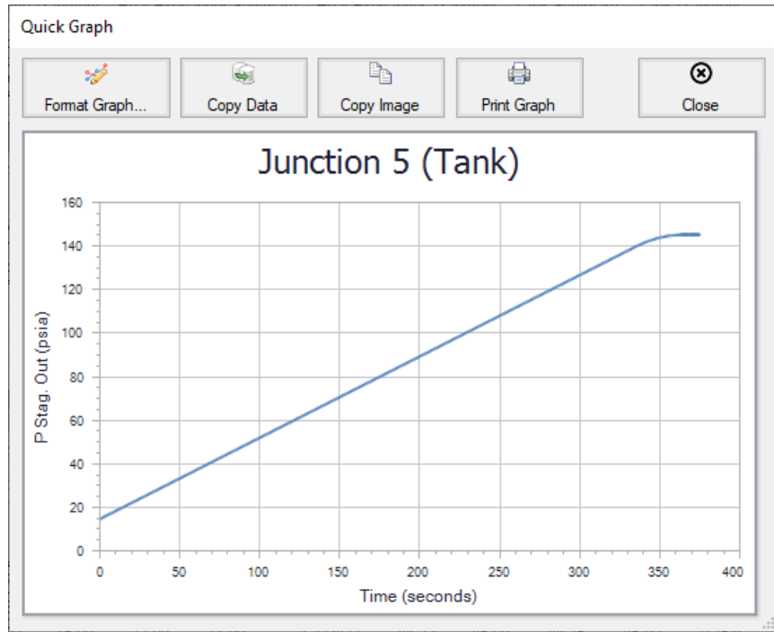
Figure 5.20 Quick Graph Plot of J5 Tank pressure
