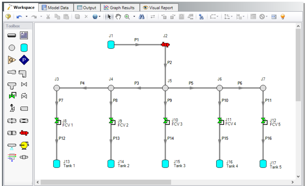
Figure 4.1 Layout of the pipe system for the Natural Gas Burner System Example
