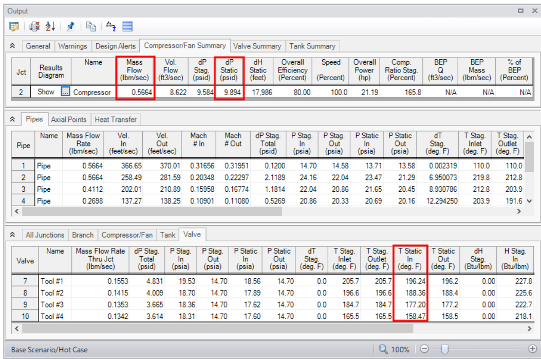
Figure 3.9 Output window for the Hot Case scenario
