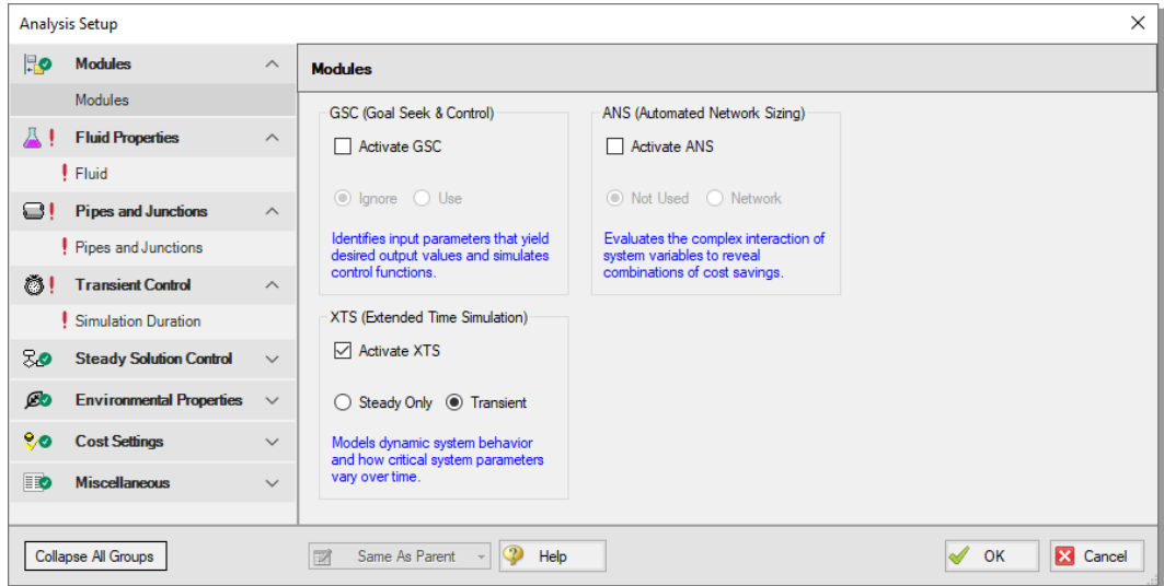
Figure 5.10 Activating the XTS module and setting the simulation type to Transient
