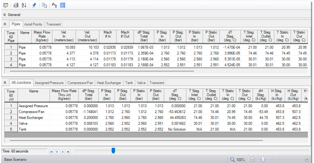
Figure 5.22 Pipe and Junction transient data at Time = 60 seconds
