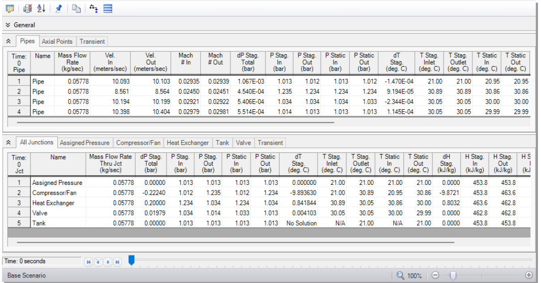
Figure 5.21 Pipe and Junction transient data at Time = 0 seconds
