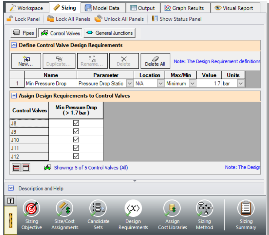
Figure 4.5 Control Valve Design Requirement defined for the primary case
