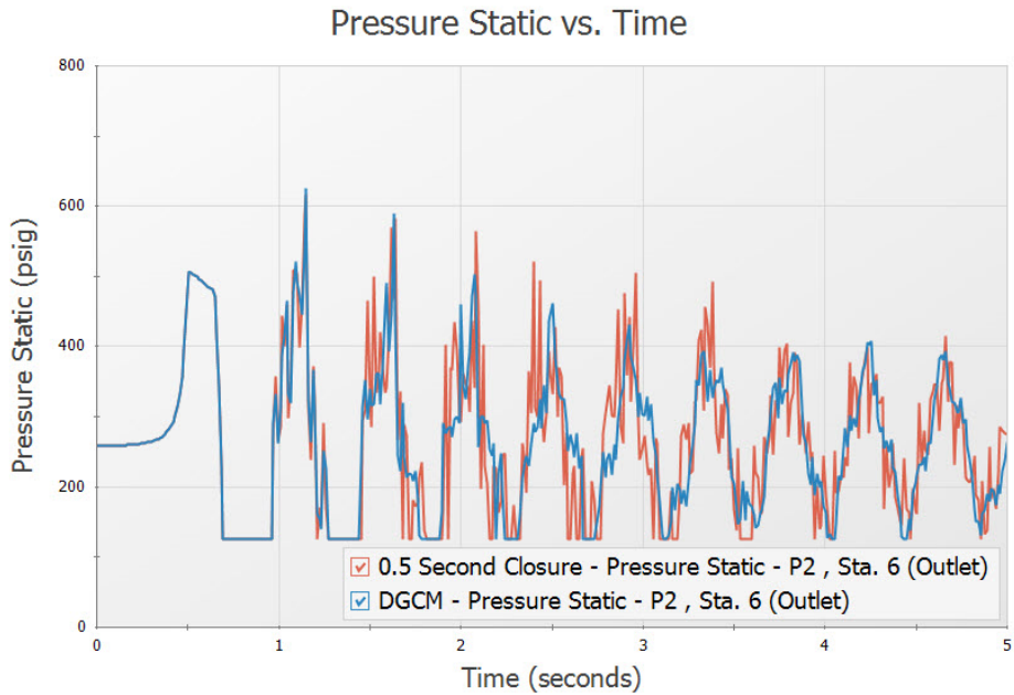
Figure 9: Multi-scenario graph comparing DVCM and DGCM results at the valve inlet for the 0.5 Second Closure scenario
